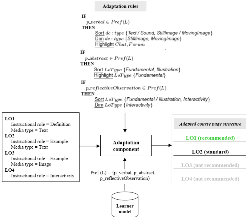
Figure 4. Automatic generation of an adapted course page for a student with preferences towards Verbal perception modality, Abstract concepts and Reflective observation
